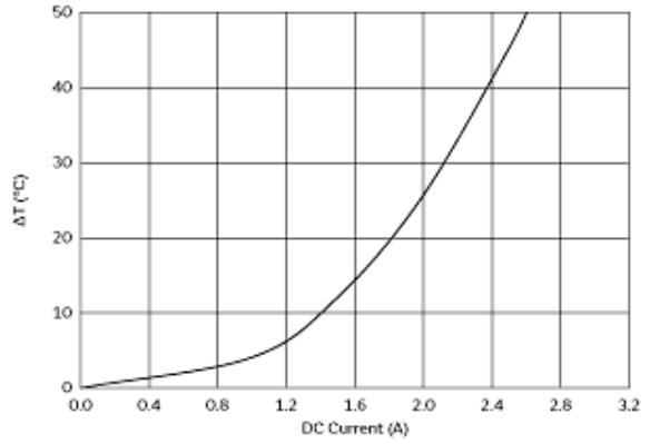
Temperature Increase Characteristic
